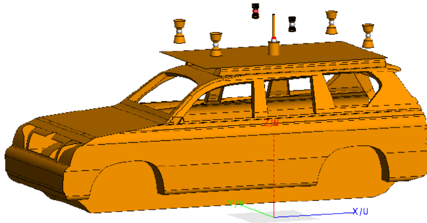
Figure 7: Simulations offer a relatively inexpensive option to investigate the coupling between antennas that are co-located on structures like vehicles or masts. An added advantage is that the effect of the structure itself can also be investigated.
