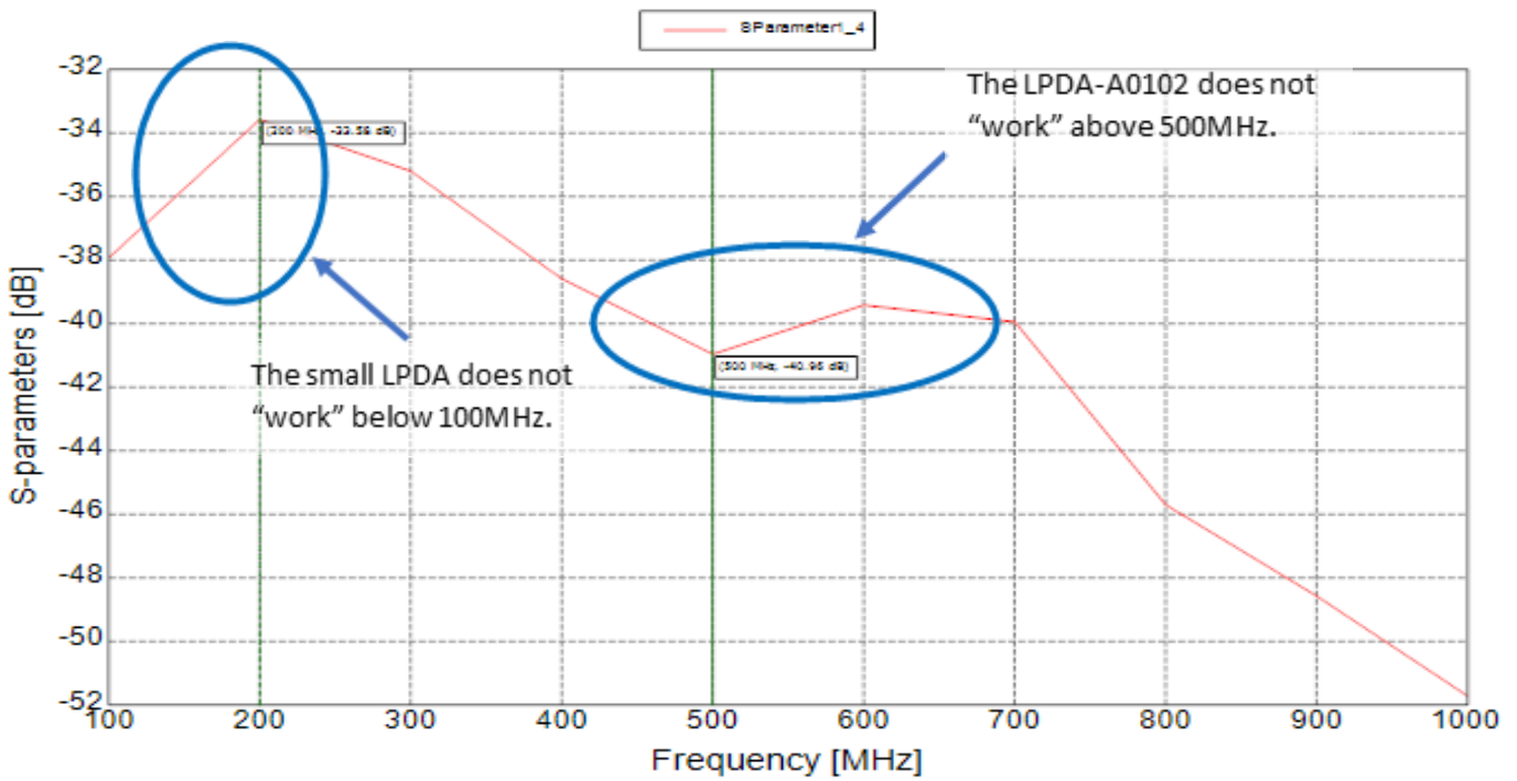
Figure 6: There is significant coupling between the two antennas outside of the overlapping frequency bands of the two antennas.
