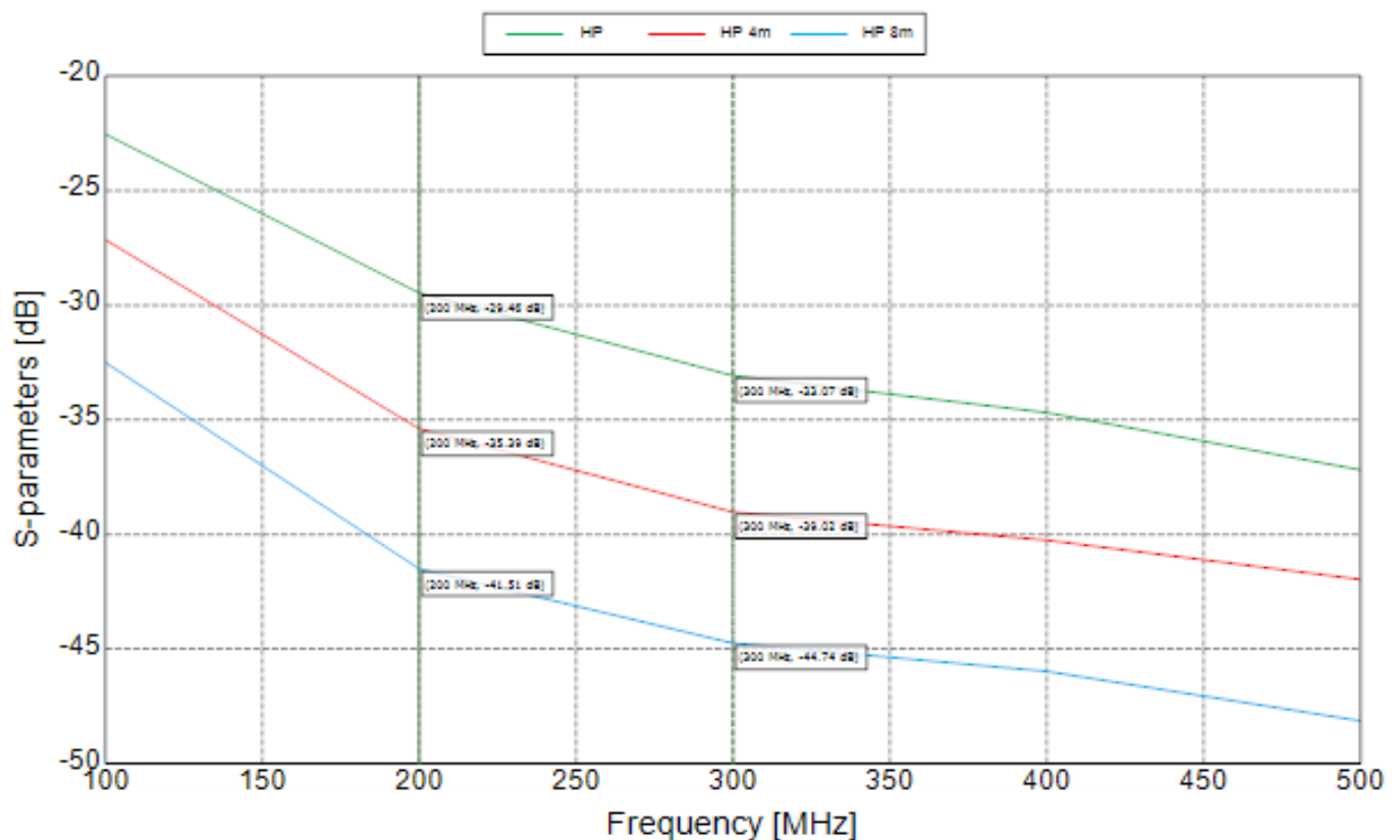
Figure 4: Coupling ( S_{21} ) between antennas that are spaced 2m, 4m and 8m apart. Every time the spacing doubles, another 6dB of isolation is achieved.
