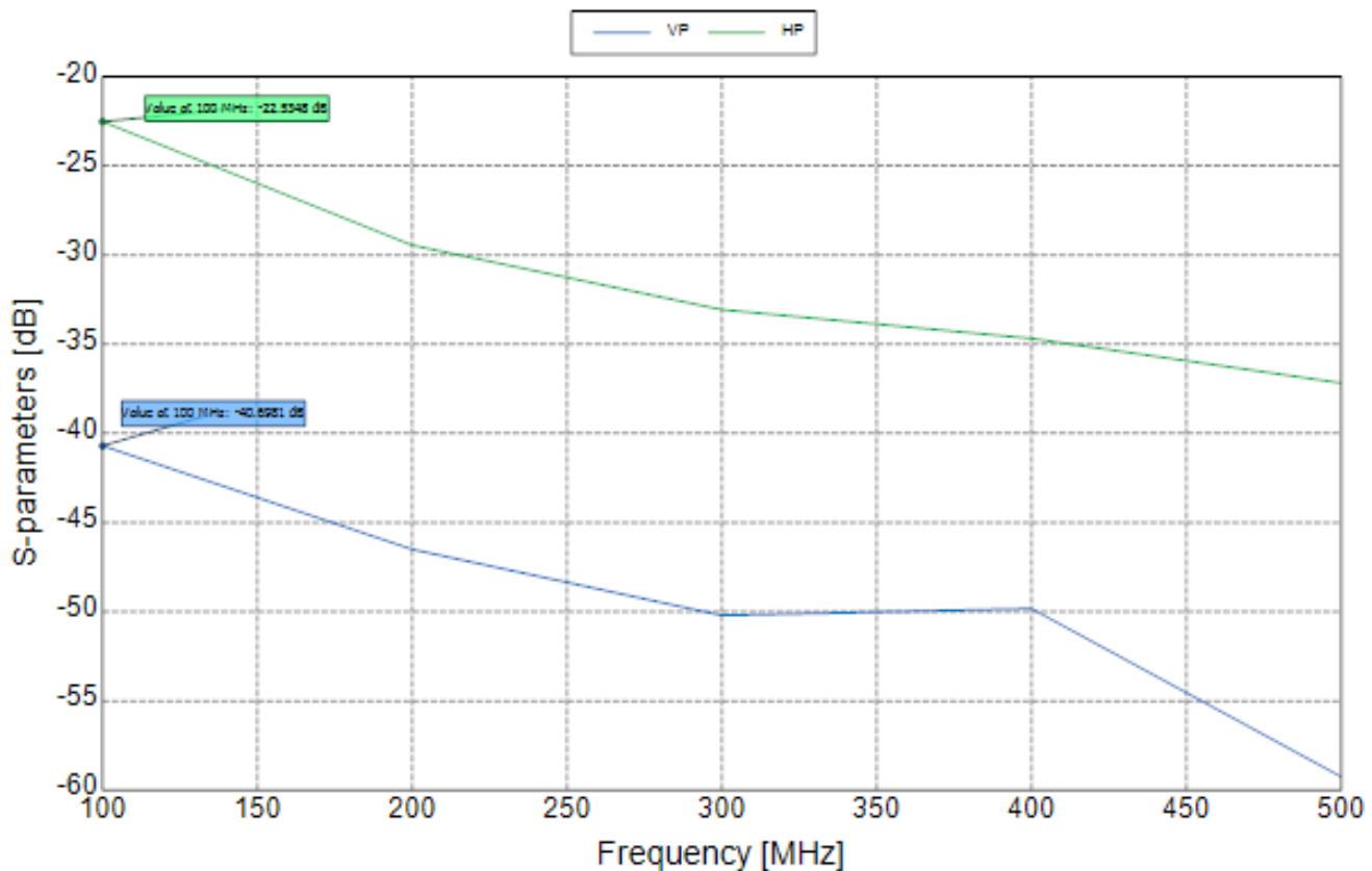
Figure 3: The coupling ( S_{21} ) between the two VP antennas (blue) is much lower (-40.7dB) compared to that of the two HP antennas (green) (-22.5dB).
