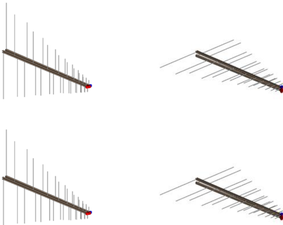
Figure 2: Two antennas mounted in vertical polarisation (left) vs horizontal polarisation (right).
